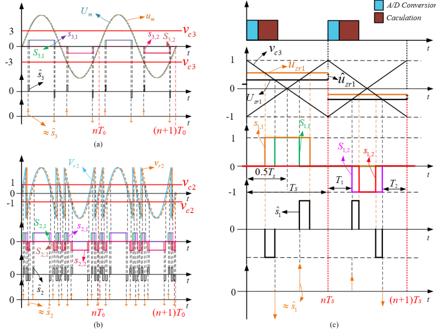
Fig. 4 Diagram of the hybrid modulation with small disturbance: (a) the high voltage Cell (Cell3) (b) the medium voltage Cell (Cell2) (c) the low voltage Cell (Cell1)
